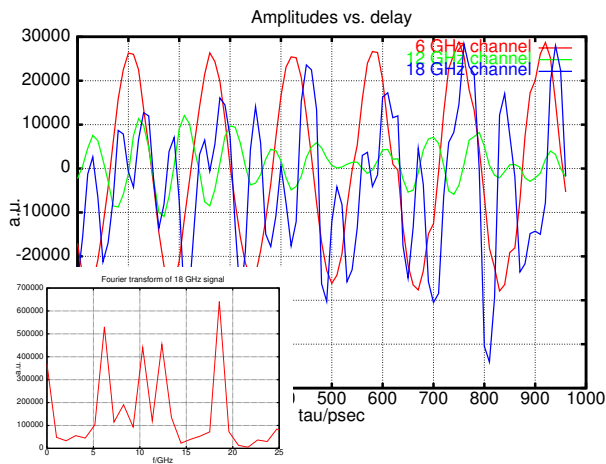
Figure 4: Amplitudes versus delay setting (Bunch current 0.2 mA). In the insert Fourier transform of the 18 GHz output.
