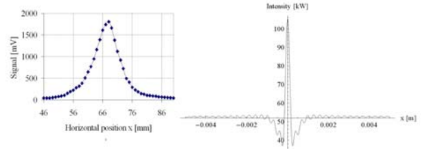
Figure 9: Left side: Horizontal scan of CTR in the focal plane of set-up B. The peak field strength exceeds 3 kV/cm. Right side: Simulated intensity pattern on the EO-crystal (acc. to eq. 1), assuming 3 optical elements with \nu_{\text{cutoff}} = 300 GHz and the same electron distribution as assumed for fig. 6 with 0.5 nC.
