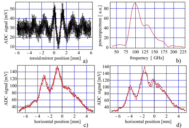
Figure 4: a) Phase scan showing the interference between the two beam paths; b) resulting power spectrum. Horizontal intensity distribution measured in the focal plane of the interferometer; c) at the fixed phase of interferogram minimum; d) at toroid mirror position 0 mm.
